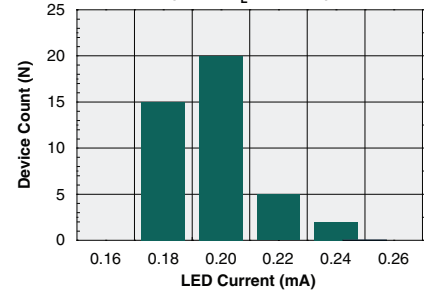
Typical I_F for Switch Dropout (N=50, I_L=400\text{mA} )
